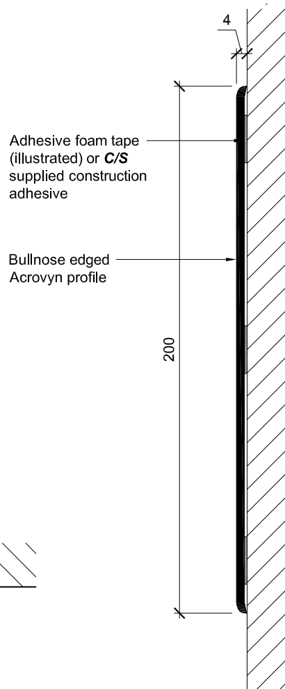
TP200 Side Elevation
