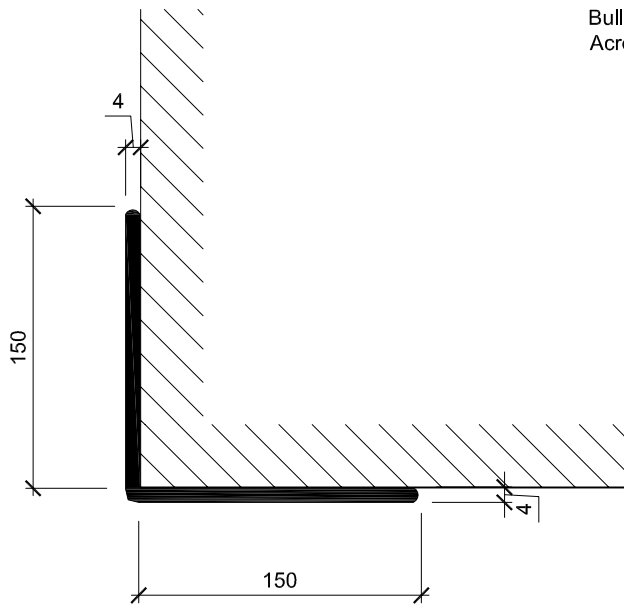
TP200 Corner Protection Plan View
