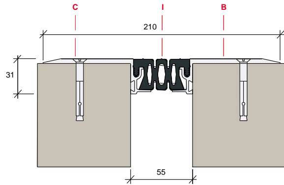
RLO-50/31. Heavy Duty Seal floor-to-floor joint cover.
